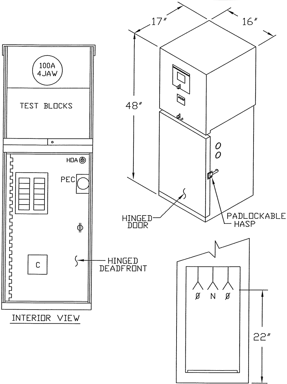
REAR LANDING DETAIL, COVER REMOVED
